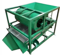
Grain Sieve Machine - Electric 2.2KW 500kg/hr
